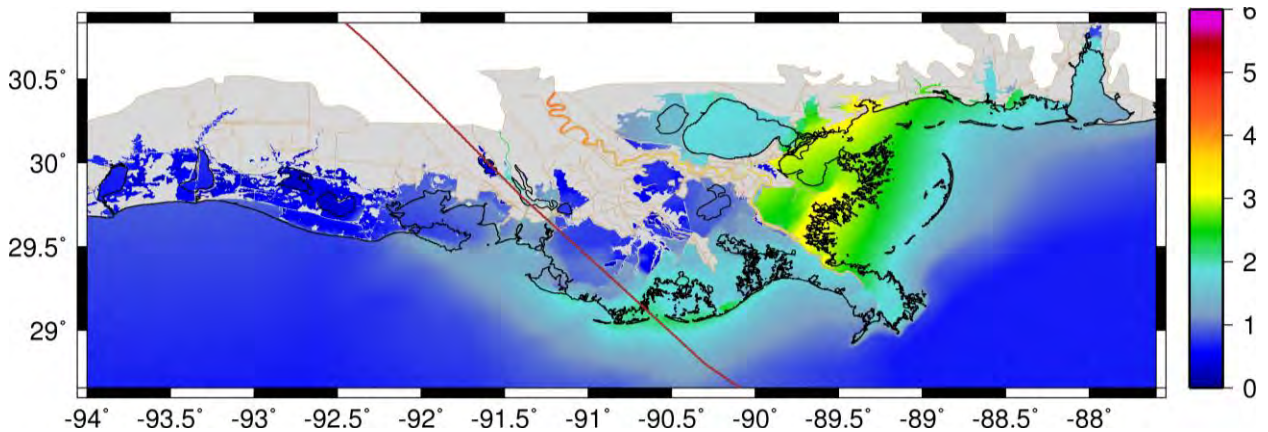
Figure 22: Maximum Storm Surge Elevation (m, NAVD88) During the 2017 CPRA Hurricane Gustav Simulation. Storm track shown in brown.
